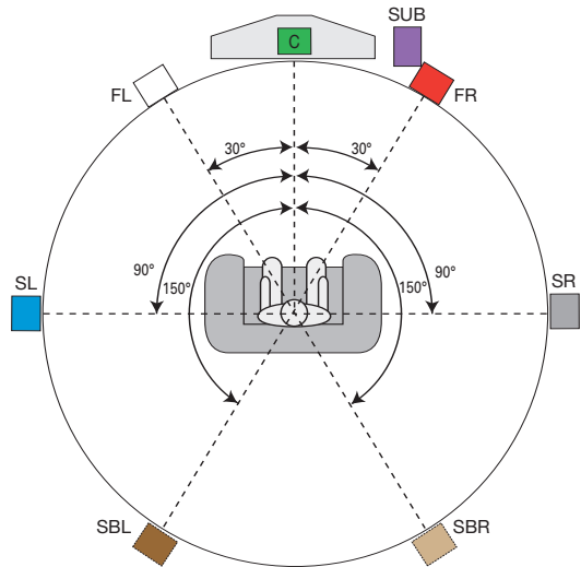
Figure 16 – Speaker Placement (7.1-Channel System)
